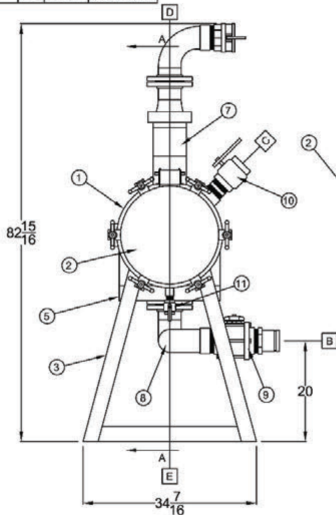
END VIEW
